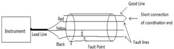
Figure 3.2.3 wiring of other-crossed fault
